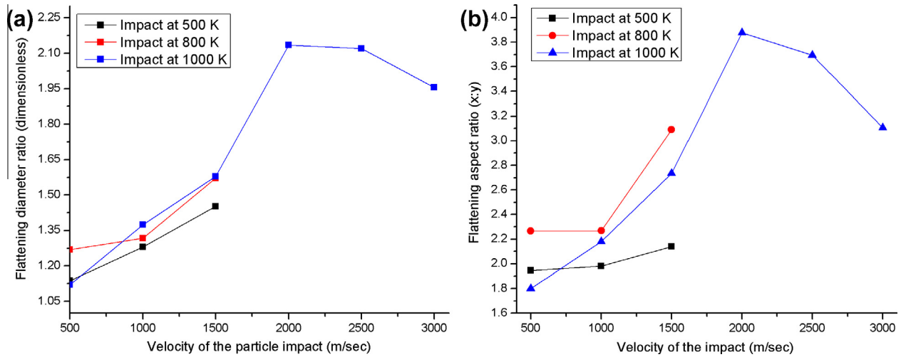
Fig. 4. Variation in the flattening ratios with respect to velocities of the particle impact when the particles were impacted at a preset temperature of 500 K, 800 K and 1000 K respectively.
