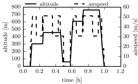
Figure 11 Training mission altitude and airspeed profiles
