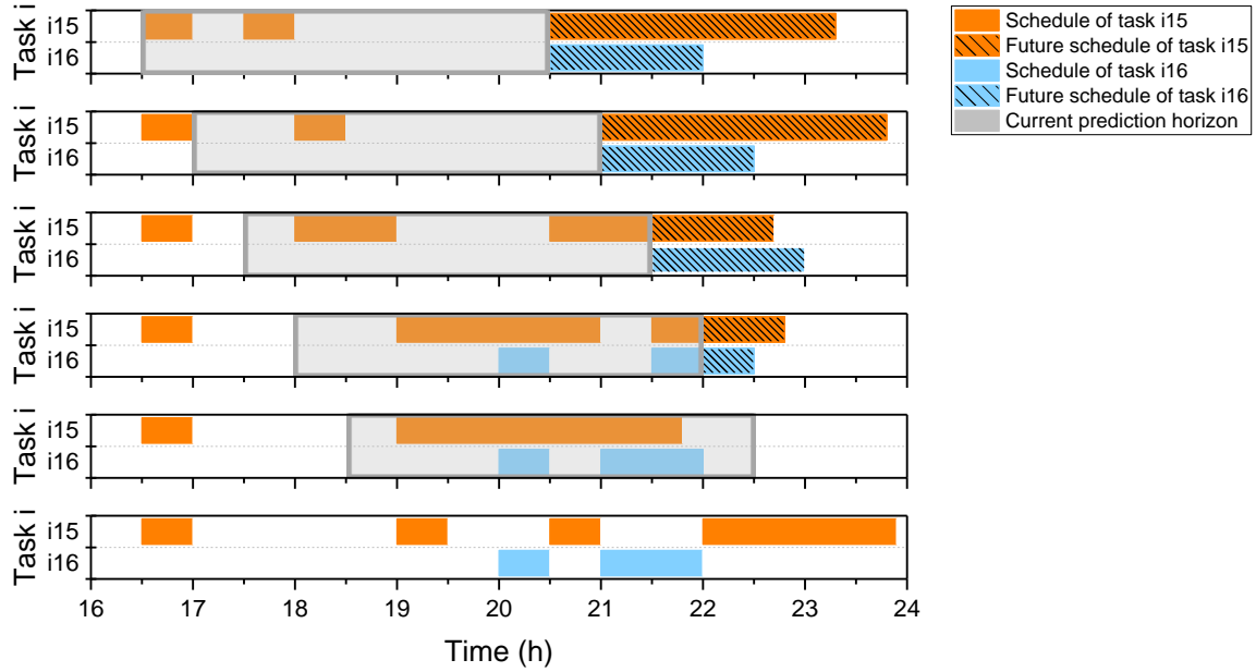
Figure 10. Evolution of scheduled tasks for 1 home and prediction horizon of 4 hours for different iterations. The last schedule corresponds to the final-implemented schedule.
