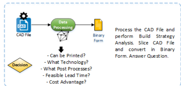
Figure 18 - AM assessment
