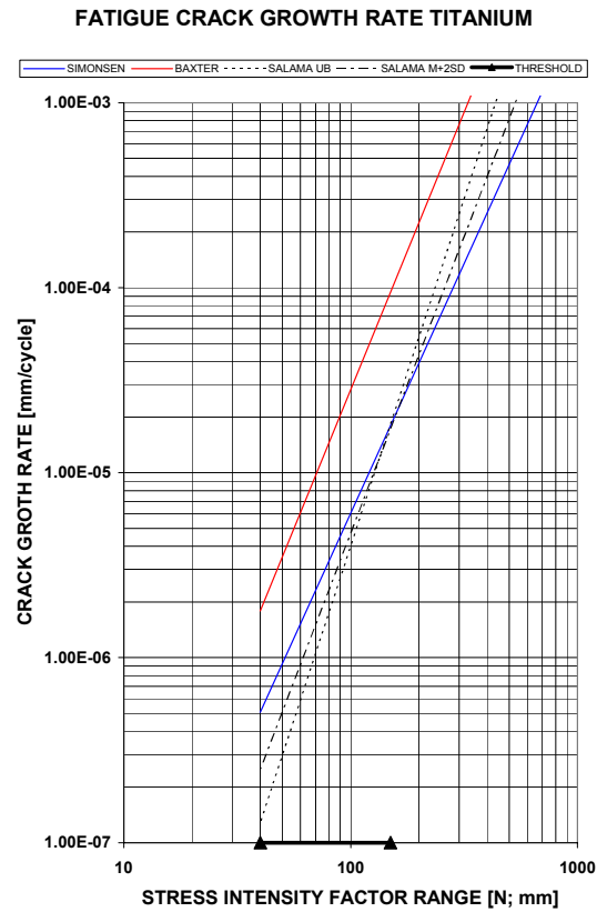
Figure 7: Illustration of fatigue crack growth curves for titanium. Fatigue crack growth thresholds are reported between 40 and 150 Nmm -3/2
