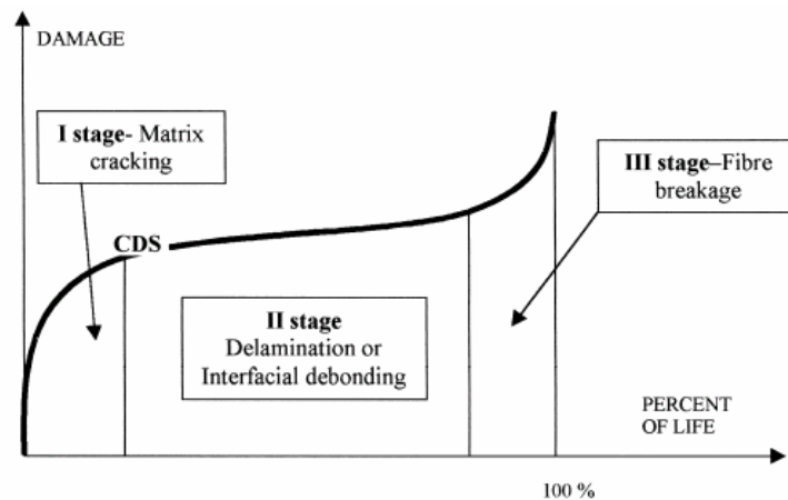
Figure 11: Development of Fatigue Damage (from Tarleja R. (1990))
