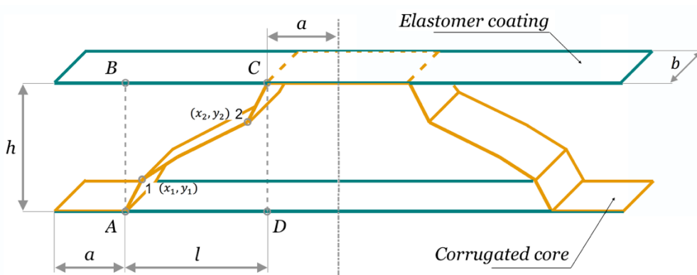
Figure 3 A unit cell of corrugation with arbitrary shape
