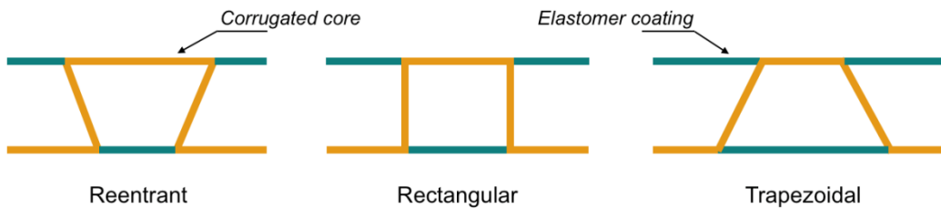
Figure 2 Three typical shapes of corrugation
