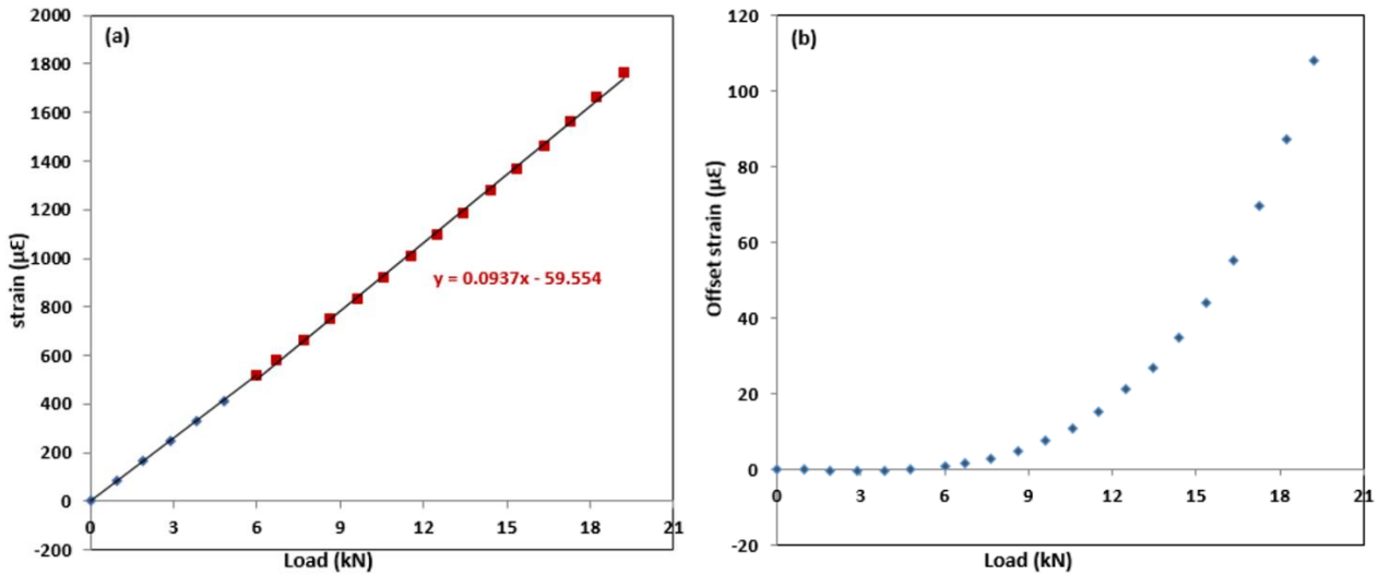
Fig.4 (a) compliance curve from the node 2mm ahead of the notch, (b) offset compliance curve from the node 2mm ahead of the notch.
