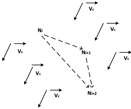
Fig. 4. Visibility algorithm demonstration.
