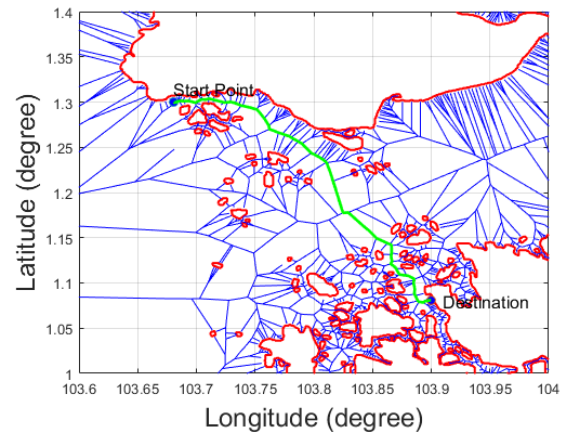
Fig. 7. Voronoi shortest path generated based on the distance weight.
