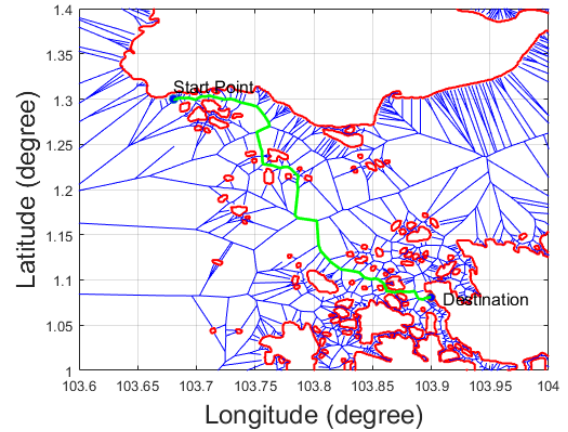
Fig. 6. Voronoi energy efficient path based on the sea current data at 2:00 hours on the 11th June 2014.
