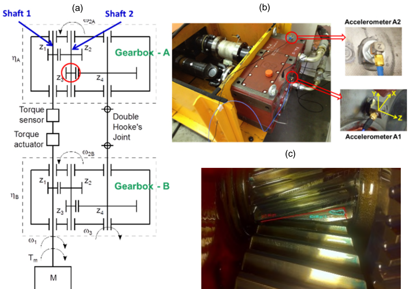
Figure 1 Test rig: Schematic Industrial gearbox with back to back gear connection
