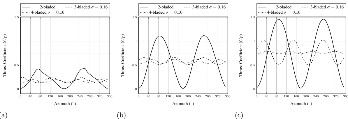
Figure 5. Instantaneous thrust coefficient at TSR = 2.02 (a), TSR = 4.6 (b) and TSR = 7.98 (c).
