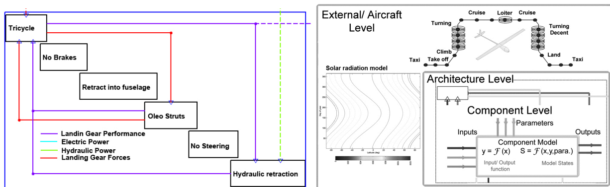
Figure 5: Analysis levels & landing gear example architecture diagram
