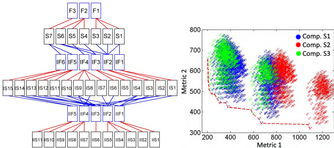
Figure 13: Function tree for the validation problem & categorized discrete space of solutions
