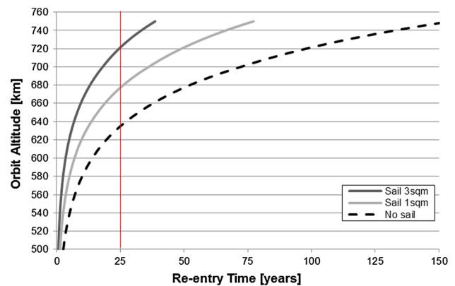
Fig. 8 Lifetime for 100 kg S/C with cross-sectional area of 1 m 2 (without sail) with different drag area. Lifetime calculations with solar average values and linear variation of density and scale height
