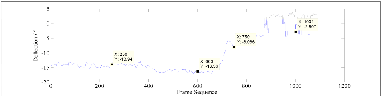
Figure 12 The wire deflection values got by manual and software
