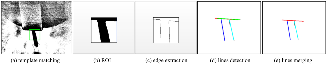
Figure 8 Procedure of the line detection process
