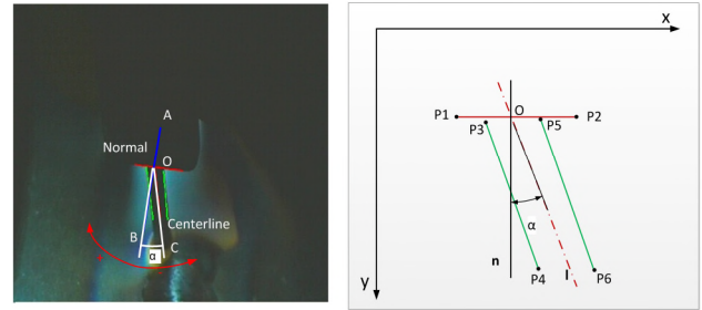
Figure 10 Diagrammatic sketch of wire deflection
