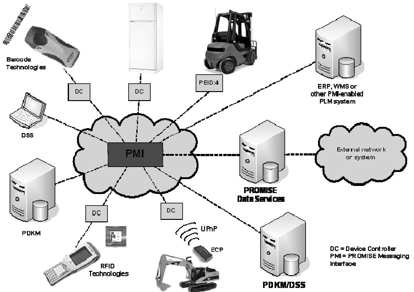
Figure 2: PROMISE Connectivity [10]
