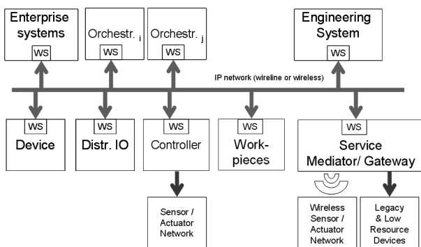
Figure 3: Service Oriented Architecture Schema
