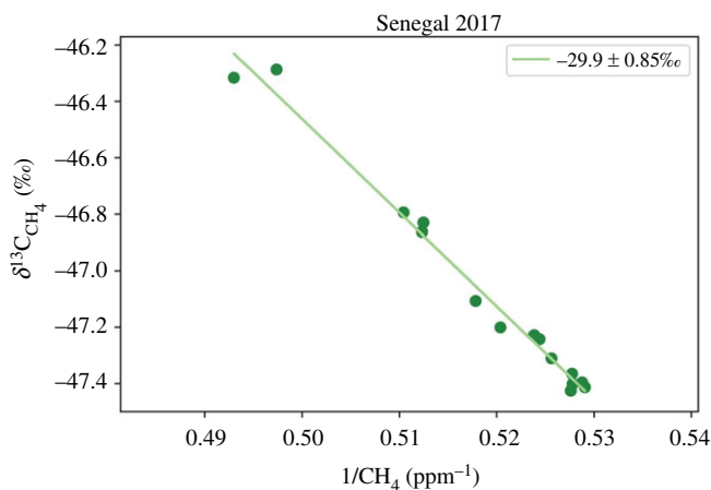
Figure 1. Keeling plot of ( 1/\text{methane abundance} ) versus \delta^{13}\text{C}_{\text{CH}_4} for isotopic measurements of samples in a fire plume on FAAM flight C005 over the Senegal Casamance region. (Online version in colour.)
