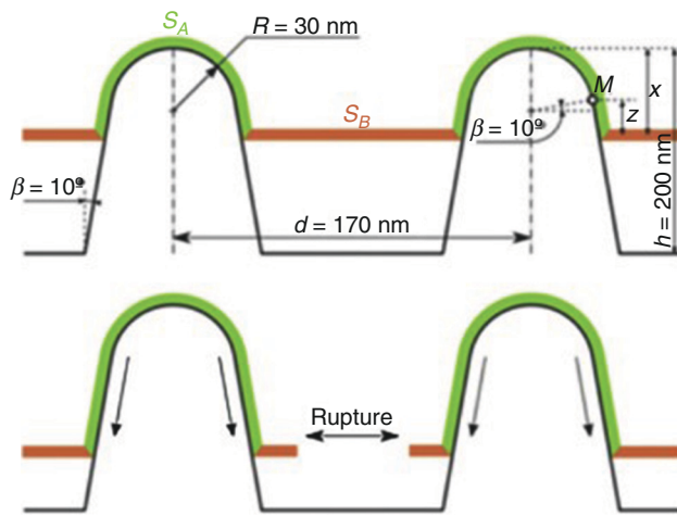
FIG. 15. Model of cicada wing and bacteria explaining rupture of bacteria. Reproduced with permission from S. Pogodin, J. Hasan, V. A. Baulin, H. K. Webb, V. K. Truong, T. H. Phong Nguyen, V. Boshkovikj, C. J. Fluke, G. S. Watson, J. A. Watson, R. J. Crawford, and E. P. Ivanova, J. of BioPhysics 104 , 835 (2013), Copyright 2013, Elsevier. 66
