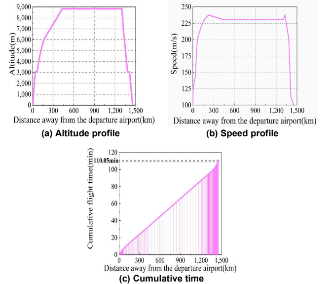
FIGURE 9. The optimized vertical profile of Objective 1.
