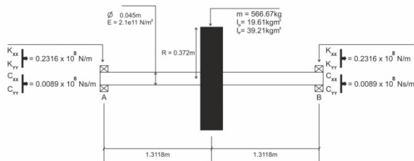
Figure 18 Simulated engine as a modified Jeffcott rotor
