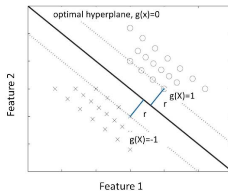
Fig. 2. SVM in the linear case.
