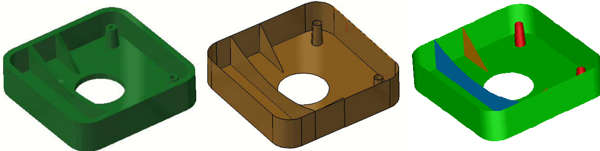
Figure 7. Simple Moulded Part, Mid-Surface Abstraction for Part and Recognised Moulding Features
