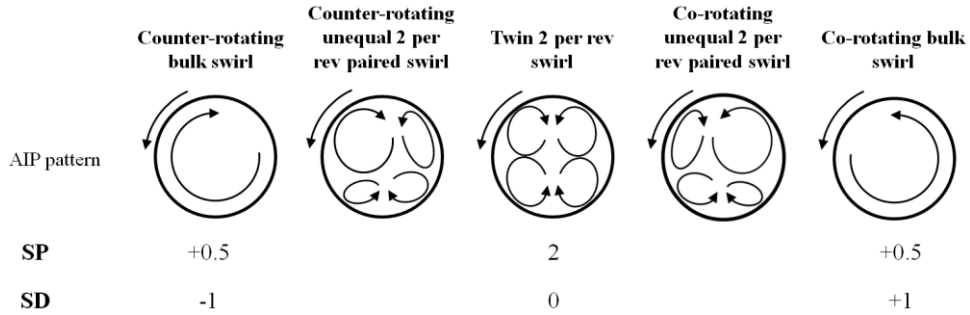
Fig. 7 Swirl Pairs and Swirl Directivity range for multiple-per-revolution swirl patterns based on SAE [4]
