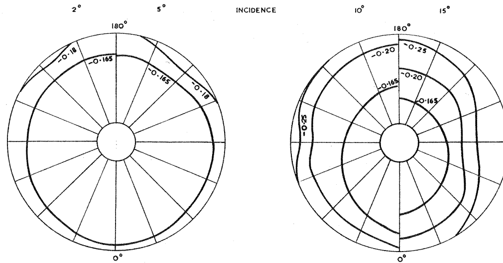
FIG 2b. BLUFF AFTER BODY.
