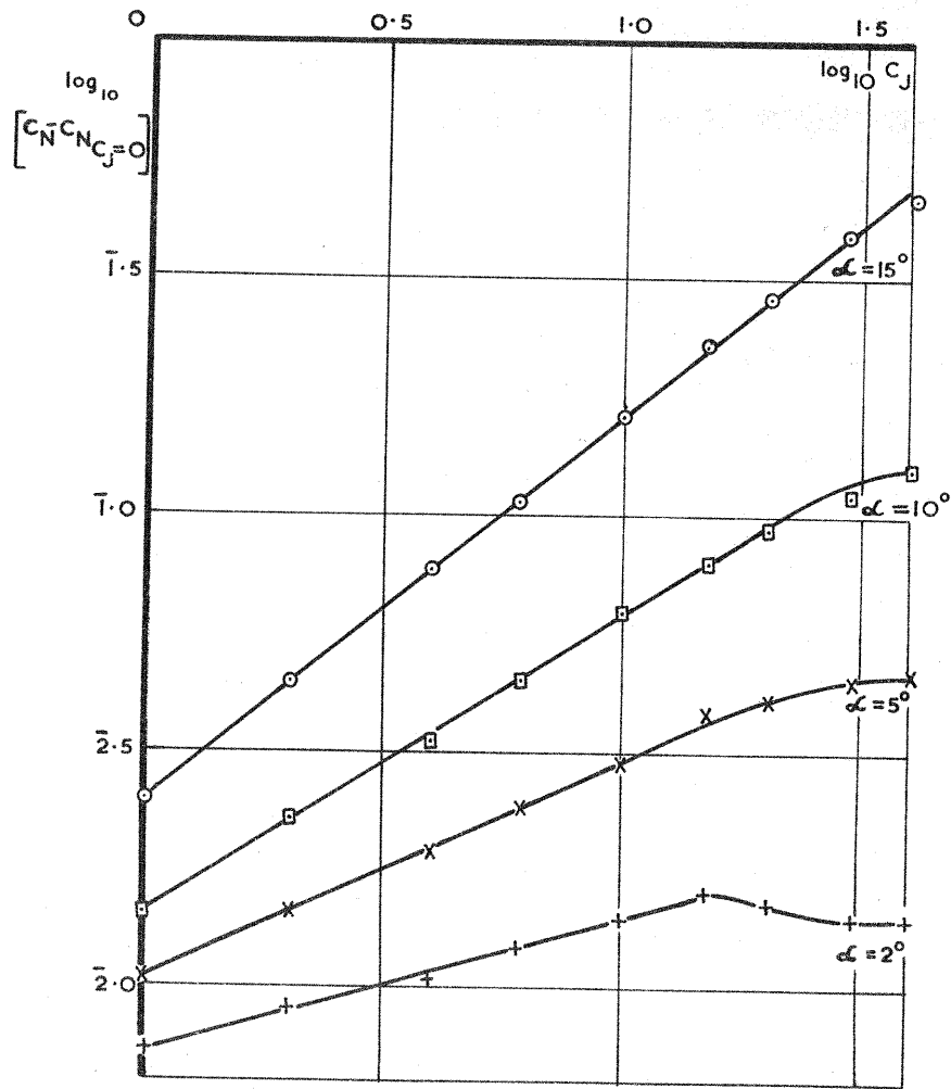
FIG. 17. DEPENDENCE OF C_N - C_N]_{C_J=0} ON C_J - BLUFF AFTERBODY
