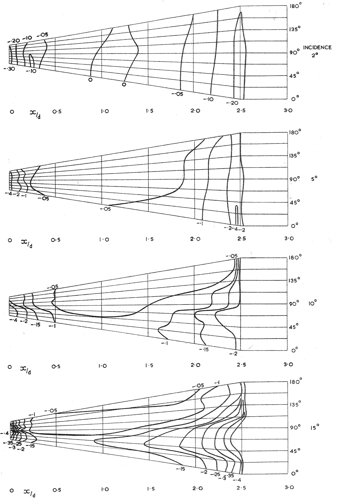
FIG. 11g. CONICAL AFTERBODY PRESSURE DISTRIBUTION C_j=20
