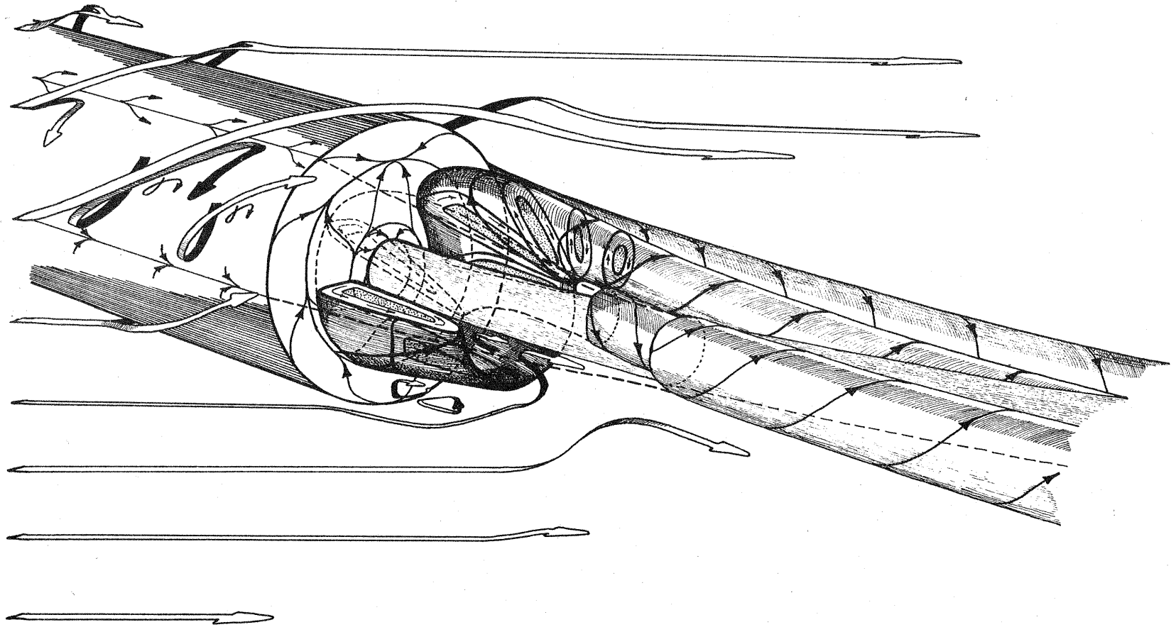
FIG. 16. THE FLOW IN THE MIXING REGION
