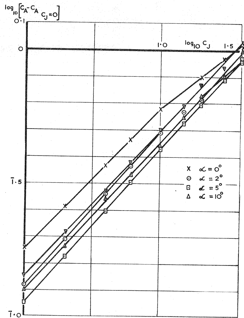
FIG. 18. DEPENDENCE OF C_A - C_A]_{C_J=0} ON C_J - BLUFF AFTERBODY
