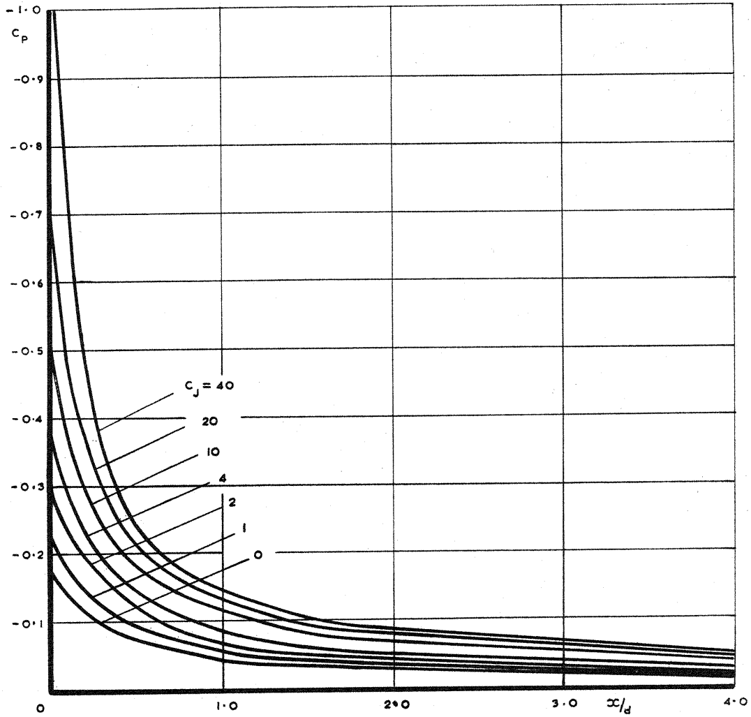
FIG. 5a. BLUFF AFTERBODY - SIDE PRESSURE DISTRIBUTION-ZERO INCIDENCE
