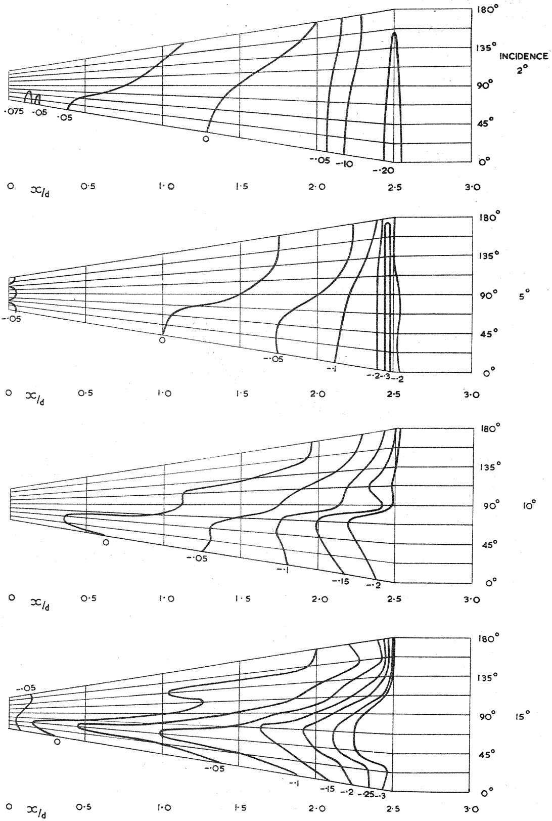
FIG. 11b. CONICAL AFTERBODY PRESSURE DISTRIBUTION C_J=0
