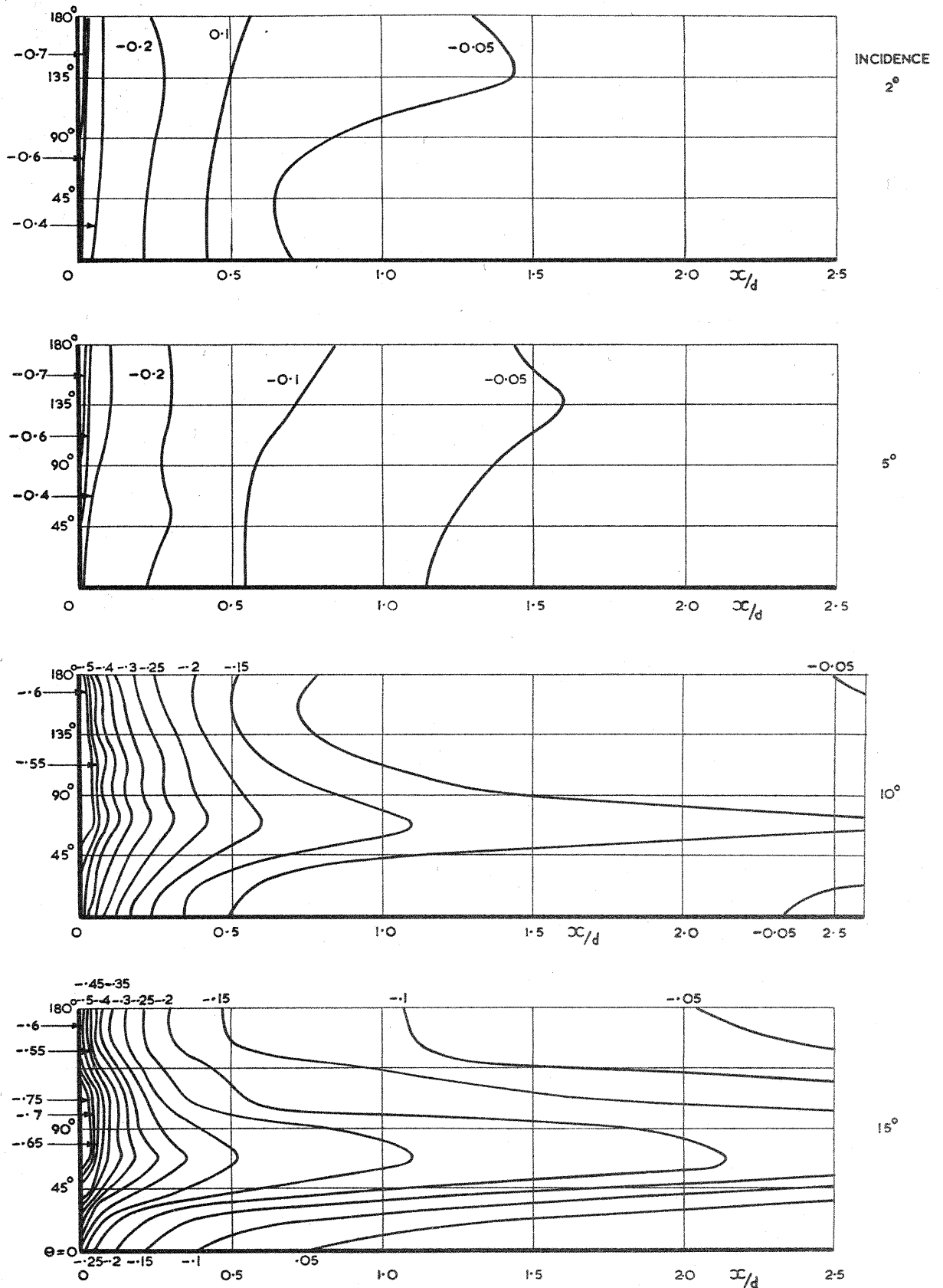
FIG. 5g. BLUFF AFTERBODY - SIDE PRESSURE DISTRIBUTION C_j=20
