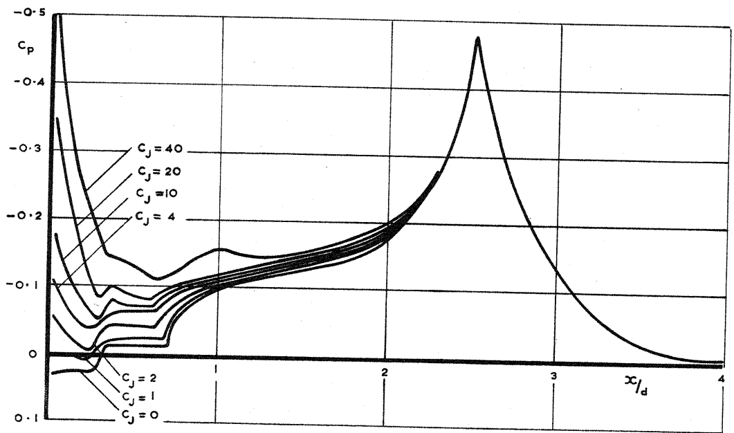
FIG. 11a. PRESSURE DISTRIBUTION ON CONICAL AFTERBODY-ZERO INCIDENCE
