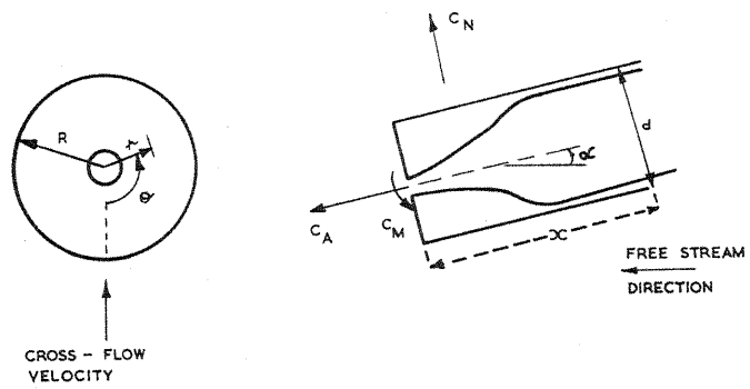
FIG. 1. DEFINITION OF SYMBOLS.
