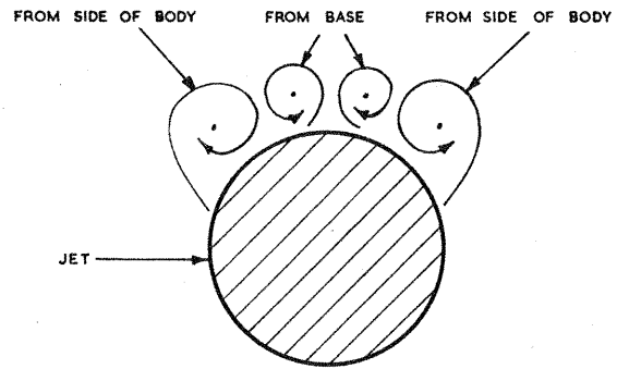
FIG. 16 a. RELATIVE POSITIONS OF THE JET & VORTICES DOWNSTREAM OF THE BASE NOT TO SCALE.
