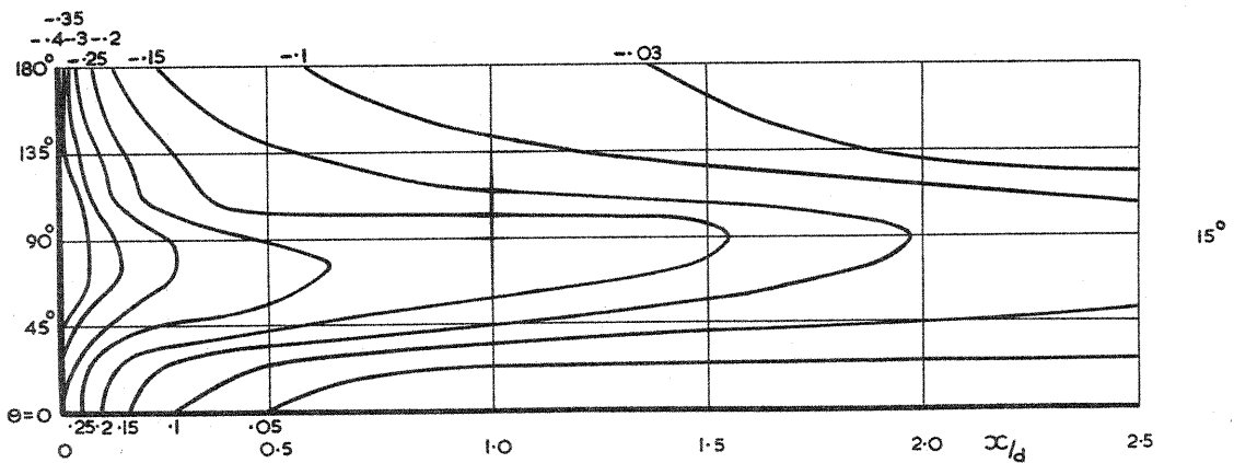
FIG. 5d. BLUFF AFTERBODY - SIDE PRESSURE DISTRIBUTION C_J=2
