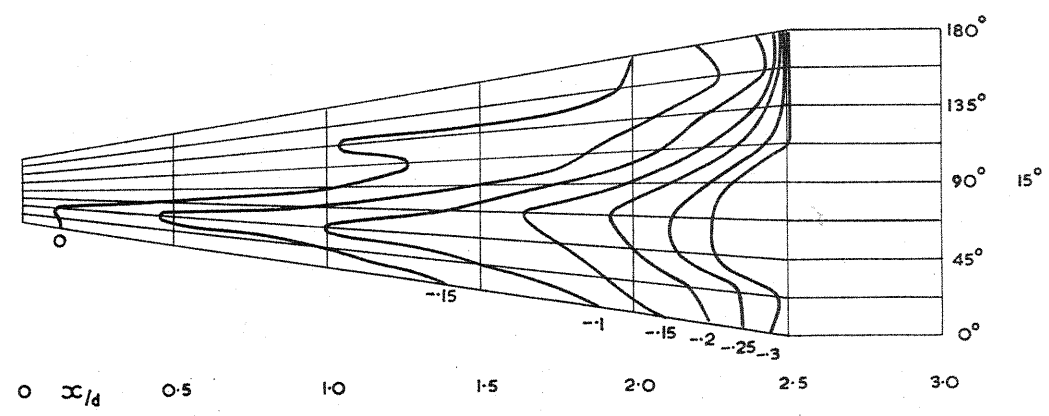
FIG. 11c. CONICAL AFTERBODY PRESSURE DISTRIBUTION C_J = 1
