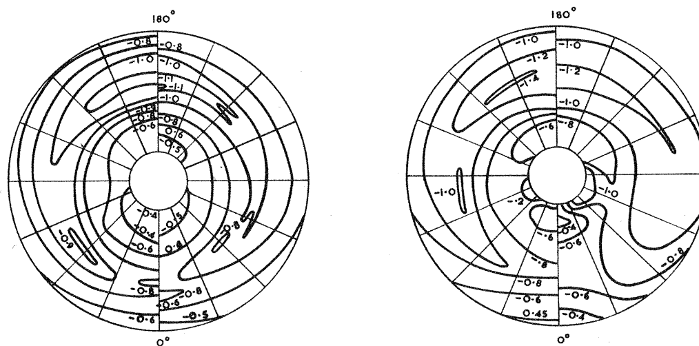
FIG. 2g. BASE PRESSURE DISTRIBUTION C_j = 20
