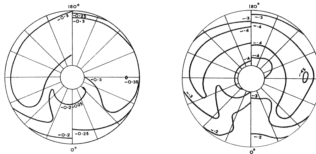
FIG. 2c. BASE PRESSURE DISTRIBUTION C_j=1
