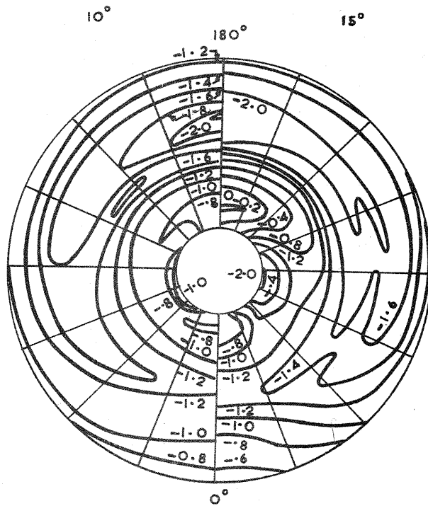
FIG. 2h. BASE PRESSURE DISTRIBUTION C_J = 40
