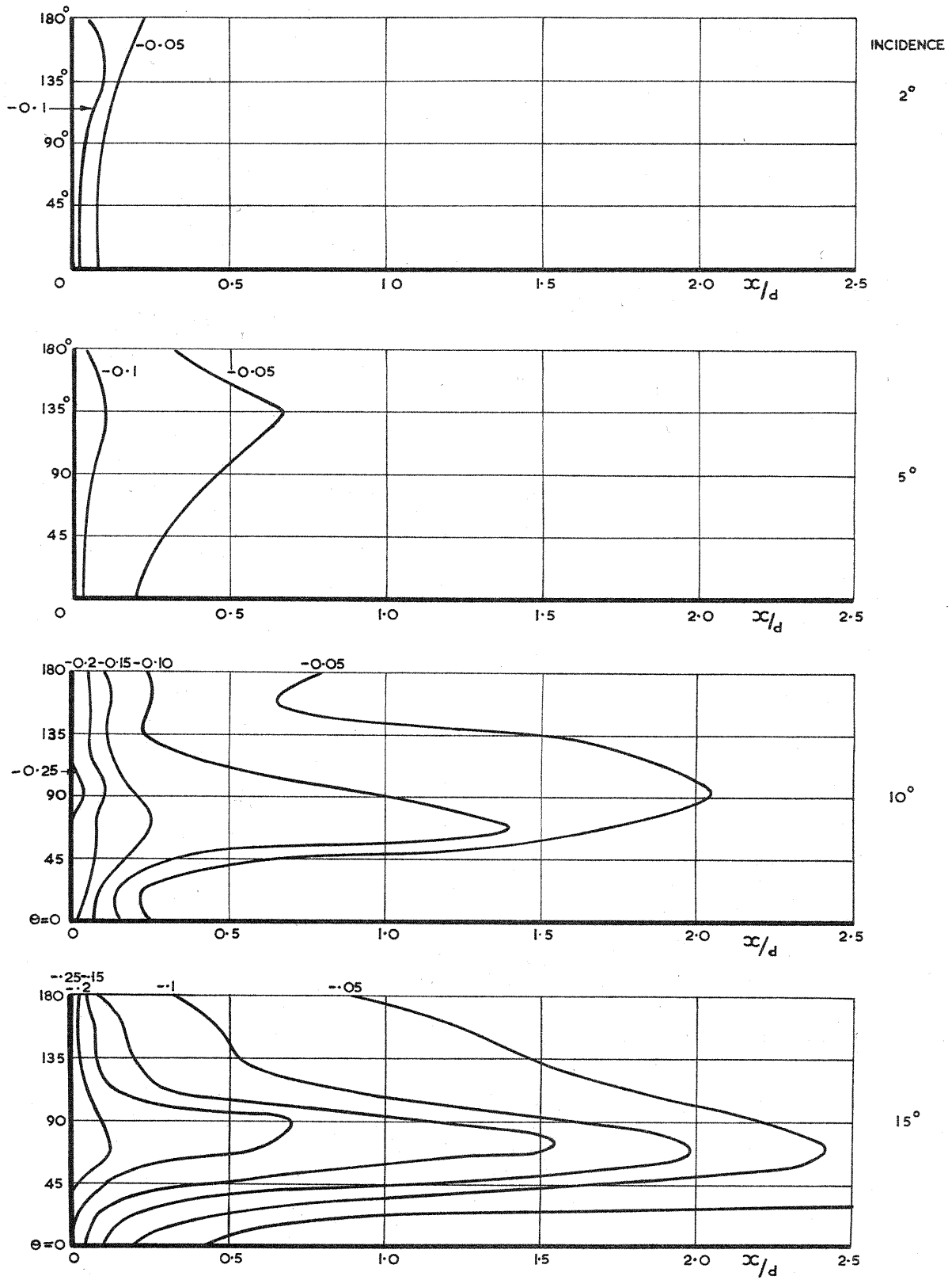
FIG. 5b. BLUFF AFTERBODY - SIDE PRESSURE DISTRIBUTION C_J = 0
