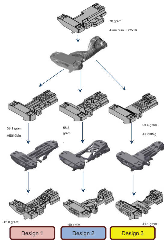
Fig.9. Roadmap optimisation of the three final designs
