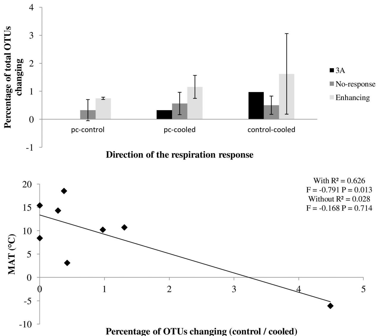
Fig 3. Number of OTUs changing (mean ± S.E) in response to time of incubation (comparing precooling vs. control) or cooling (comparing cooled vs. control soils) or both (comparing precooling vs. cooled). a) in different respiration response groups, b) linear regression between the number of changing OTUs and site MAT with or without 1H. Grey bars represent each group with standard error bars. Error bars for compensatory group were not added (n = 1). Black diamonds represent each soil (n = 8).
