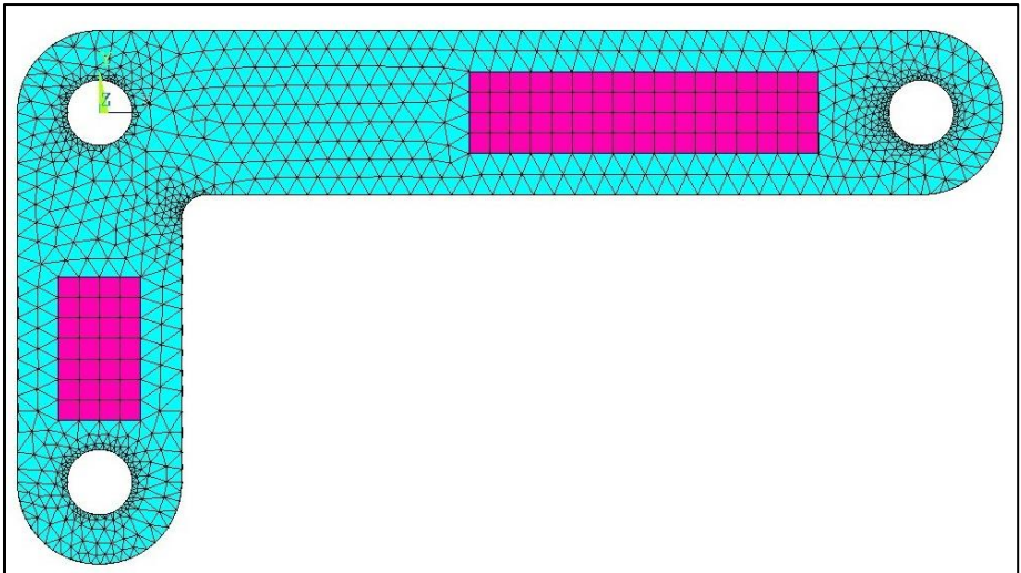
Figure 12. Modelling of the bracket using brick elements for the lattice structure.
