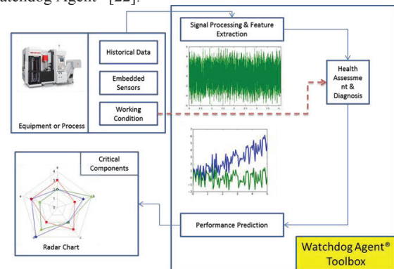
Figure 4: Flowchart of Watchdog Agent® [7]
