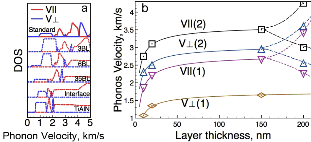
Figure 3. (a) Density of the states (DOS) of acoustic phonons and (b) dependence of Ag (TA) phonons velocity with Ag layer thickness in TiAlN/Ag coatings.
