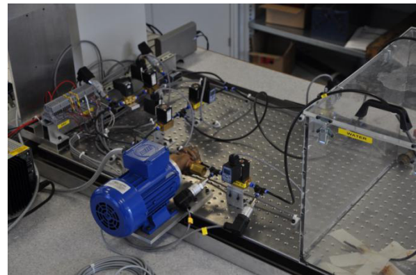
Figure 4. Fuel system test rig
