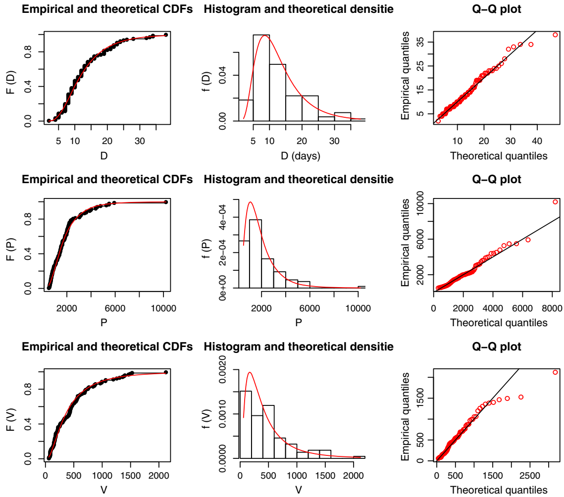
Fig. 4. Fitted distributions to the flood variables, D, P, V , are respectively shown in the 1st to 3rd rows. The 1st to 3rd columns illustrate cdfa, pdfs and q-q plots of the flood variables, respectively.
