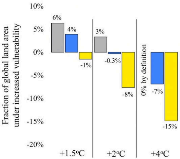
Figure 6. Global mean (across GCM) % impacts avoided relative to 4°C high adaptation challenges case (at 1.5°C, 2°C and 4°C global warming and for different levels of adaptation). Negative values correspond to benefits (positive avoided impacts) and positive values correspond to disbenefits (negative avoided impacts) compared to the GWL4-SSP3 scenario.
