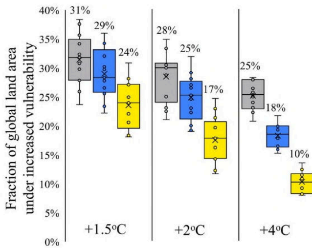
Figure 5. Global mean (across GCMs) projected changes in global population and land fraction under increased vulnerability at 1.5°C, 2°C and 4°C global warming for different levels of adaptation
