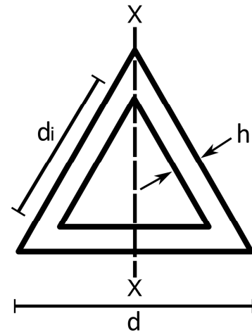
(b) Strut Cross-section
